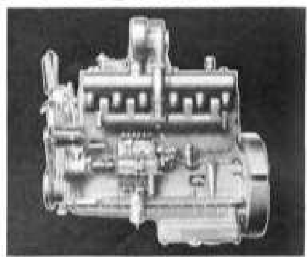
New Supercharged 6-WAKDS Diesel, with carrier-mounted turbocharger; 6-cyl., 6 1/4 x 6 1/4, 1197 cu. in., 352 max. hp.
